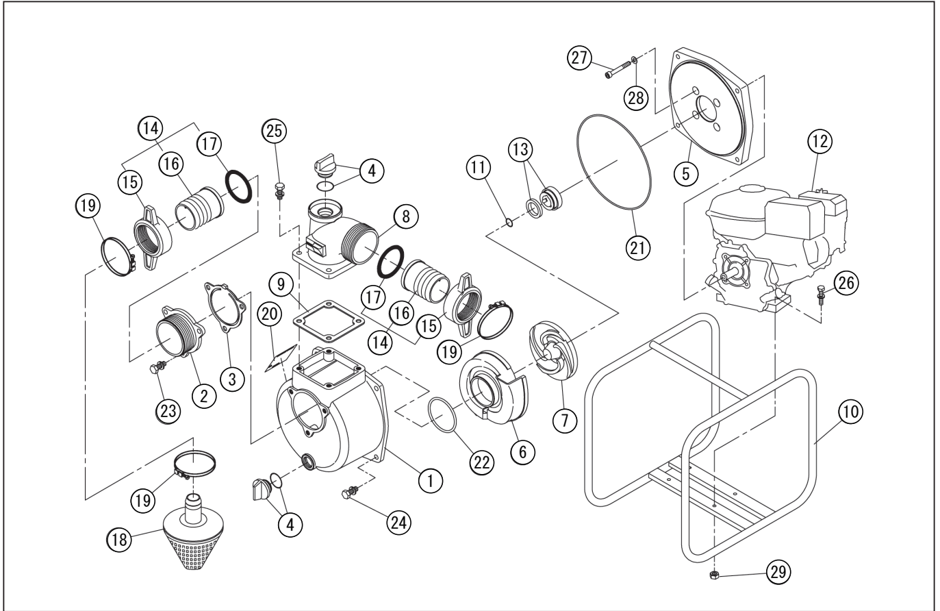
DWG No.066850611 MODEL : SEH-50X FORM : SEH-50X-BEB-1
