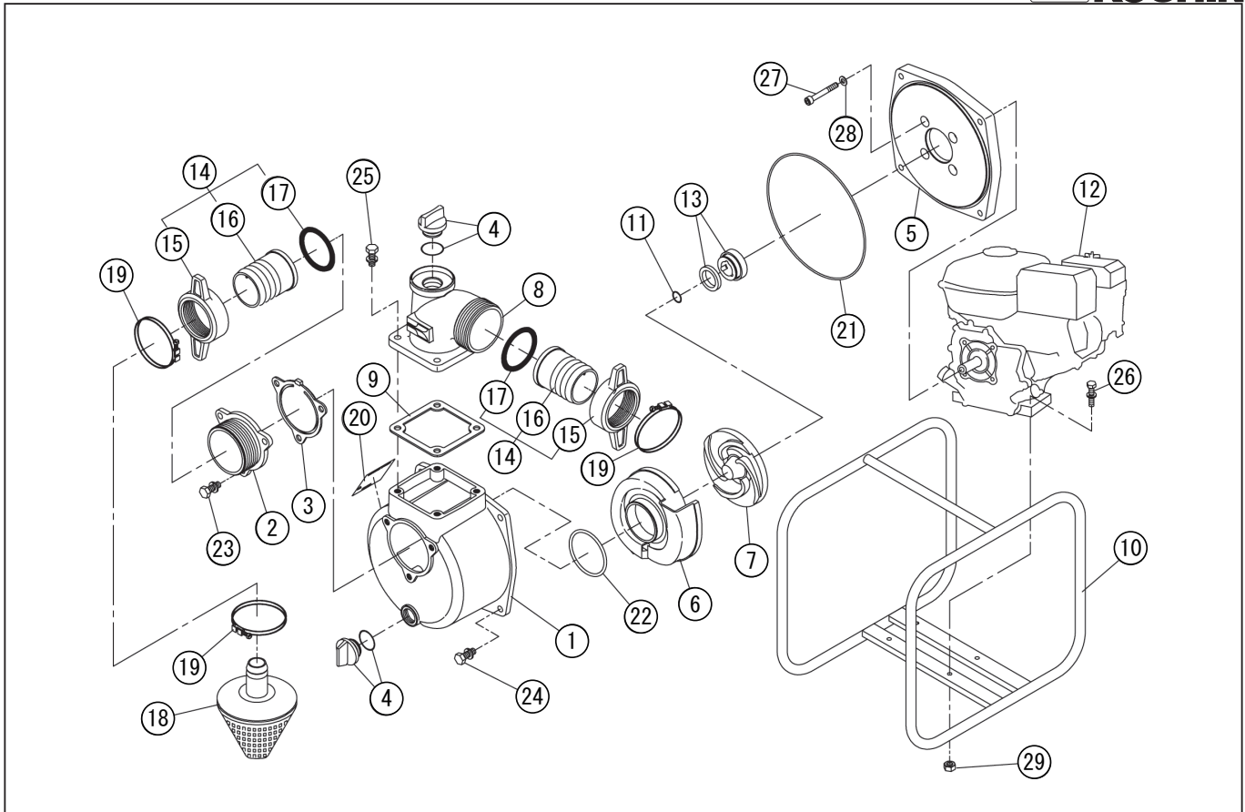
DWG No.066850911 MODEL : SEH-50X FORM : SEH-50X-BEE-1
