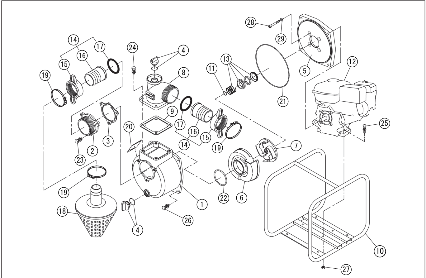
DWG No.070853003 MODEL : SEH-50X FORM : SEH-50X-BFS-0
