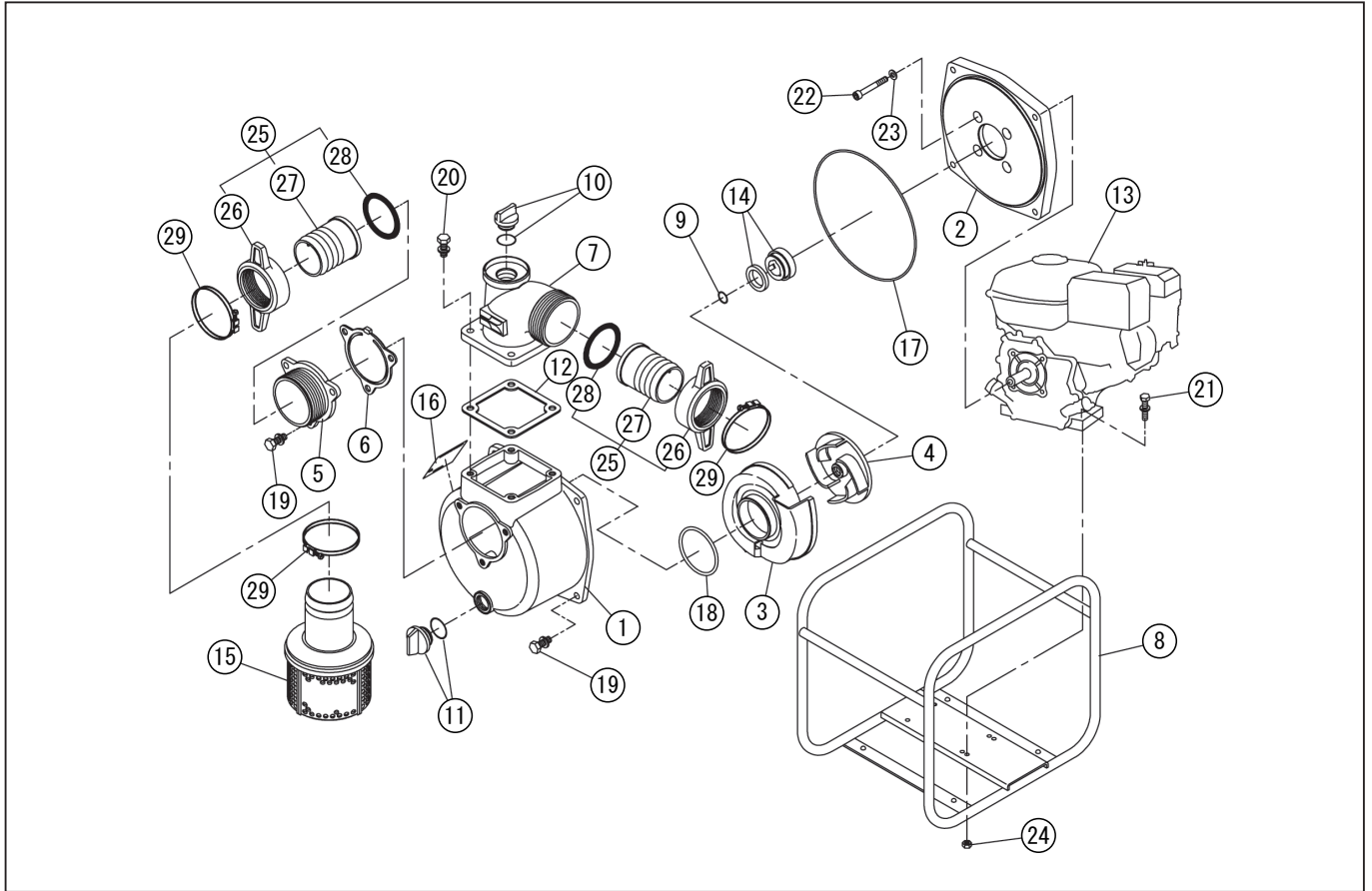
DWG No.066850107 MODEL : SEH-80X FORM : SEH-80X-BAY-2
